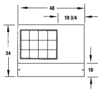
SW48-12M TOP VIEW
