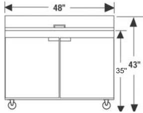
SW48-12M, 18M FRONT VIEW
