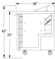
SIDE VIEW DIMENSIONS
