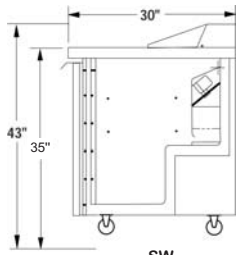
SW SIDE VIEW
