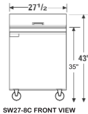
SW27-8C FRONT VIEW
