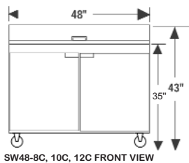
SW48-8C, 10C, 12C FRONT VIEW
