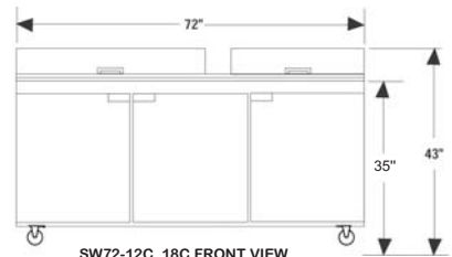
SW72-12C, 18C FRONT VIEW
